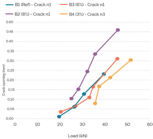
FIG. 20.5 - CRACK OPENING VS LOAD COMPARISON FATIGUE TEST - MAXIMUM CRACK OPENING COMPARISON CRACK OPENING MEASURED BY DIGITAL MICROSCOPE
