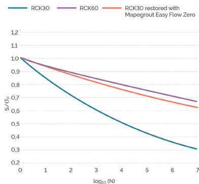
FIG. 20.2 - GRAPHIC REPRESENTATION OF S-N CURVES OF THE 3 SERIES
