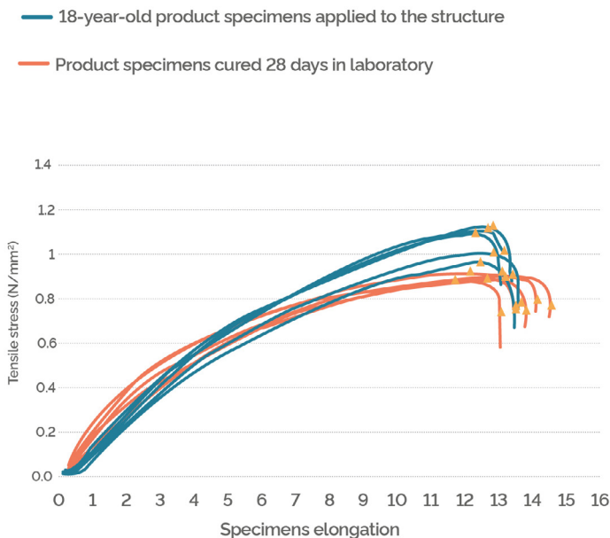
FIG. 20.7 - COMPARISON OF TENSILE STRESS AND ELONGATION VALUE BETWEEN MATERIAL SPECIMENS CURED 28 DAYS IN LABORATORY AND THOSE AGED 18 YEARS
